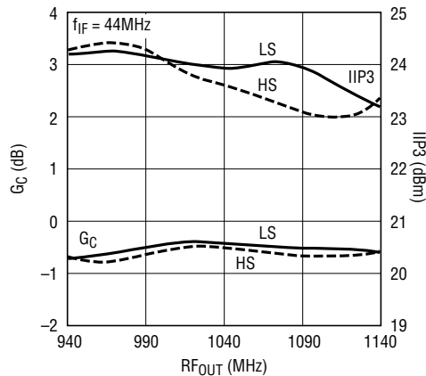
Low Side LO (LS) and High Side LO (HS) Comparison: Conversion Gain and IIP3 vs RF Frequency
