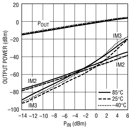
P_{OUT} , IM3 and IM2 vs Input Power
