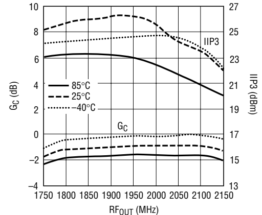
Conversion Gain and IIP3 vs RF Frequency
