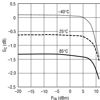
Conversion Gain vs Input Power
