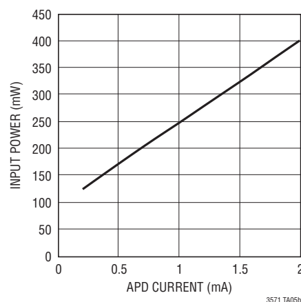
Input Power vs APD Current
