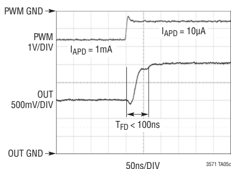
Transient Response on Input Signal Falling Edge (1mA to 10μA)
