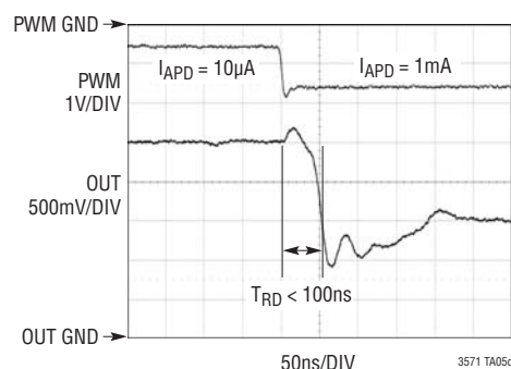
Transient Response on Input Signal Falling Edge (10 \mu A to 1mA)
