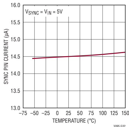
SYNC Pin Current
