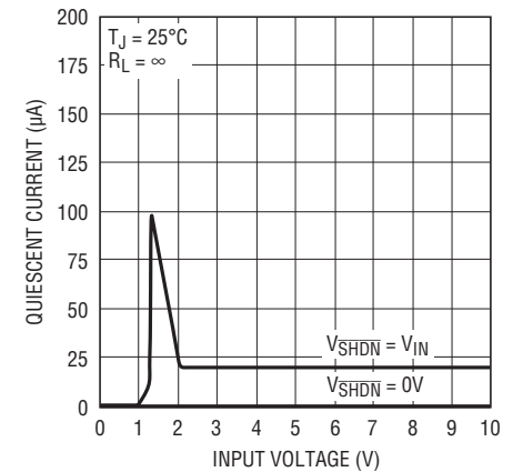
LT1761-2 Quiescent Current
