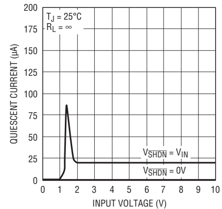
LT1761-1.8 Quiescent Current
