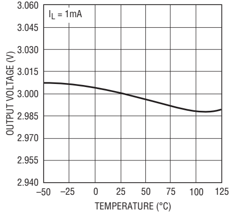
LT1761-3 Output Voltage
