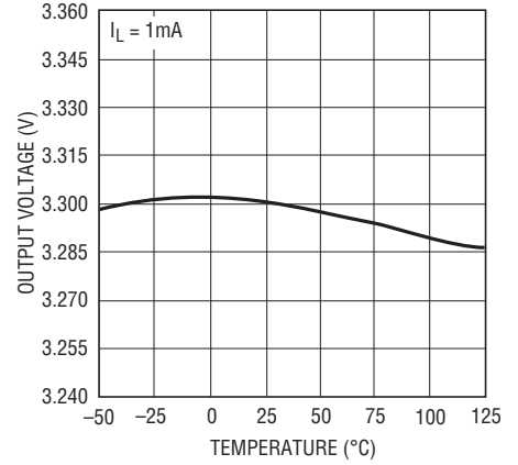
LT1761-3.3 Output Voltage
