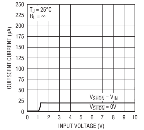
LT1761-1.2 Quiescent Current
