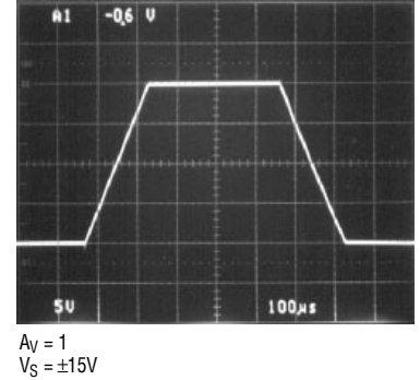
Large-Signal Response V_S = \pm 15V
