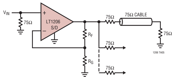
Distribution Amplifier
