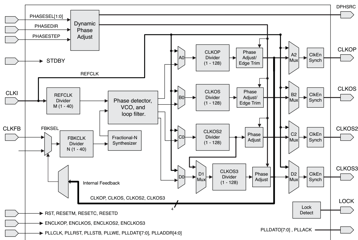
Figure 2-7. PLL Diagram
