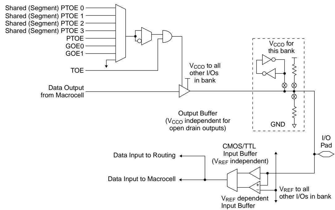
Figure 8. I/O Cell
