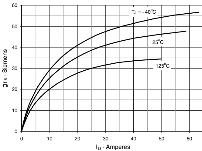
Fig. 9. Transconductance
