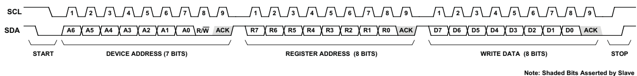
Figure 23. I 2 C Write Operation
