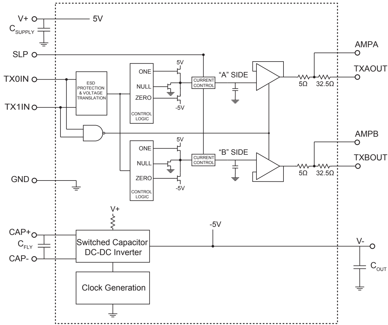
Figure 1. HI-8592 Block Diagram
