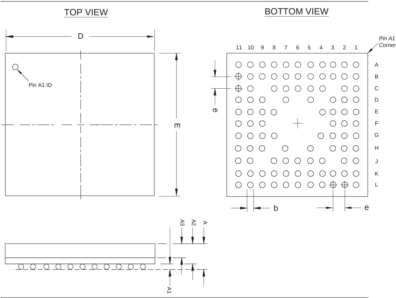
Figure 7-3. 100-Pin Micro FineLine BGA Package Outline
