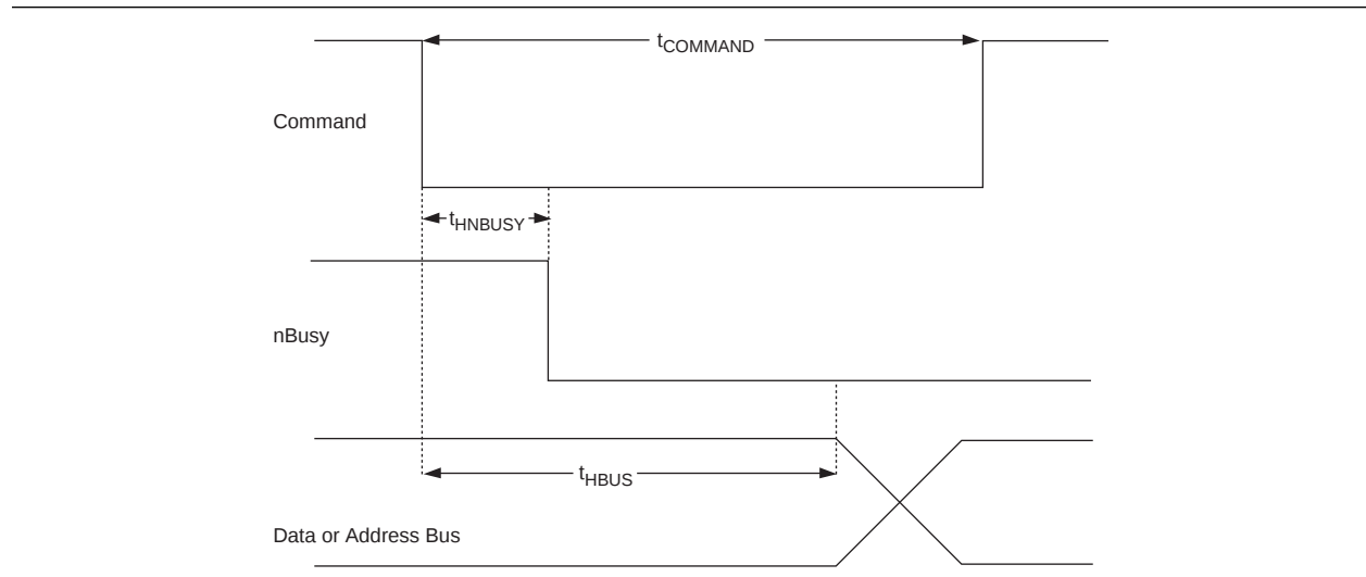
Figure 9-40. Parallel Interface Timing Waveform
