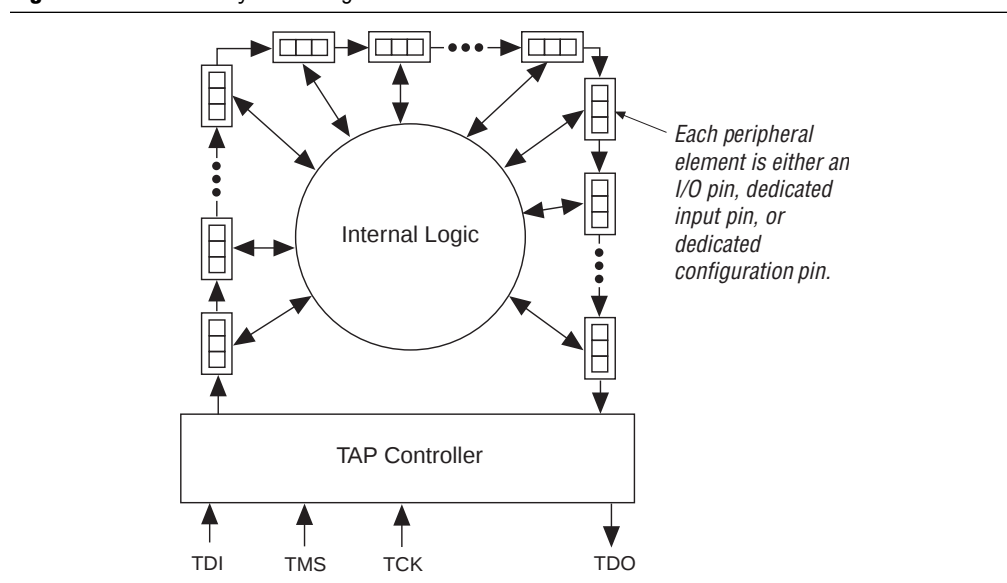
Figure 13-3. Boundary-Scan Register
