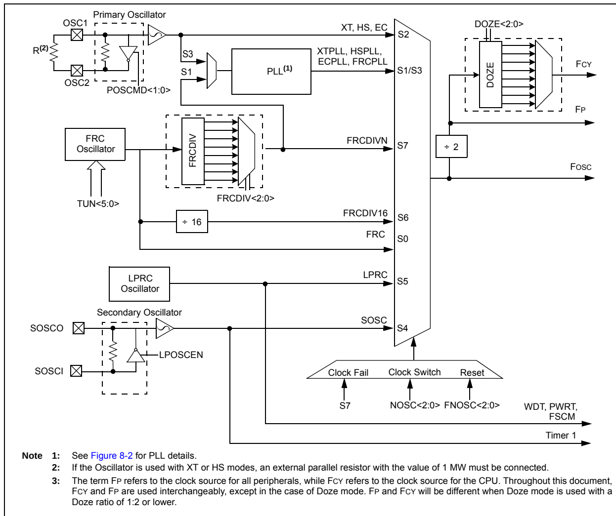
FIGURE 8-1: dsPIC33FJ12GP201/202 OSCILLATOR SYSTEM DIAGRAM
