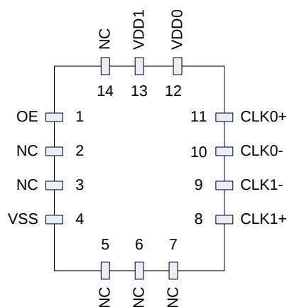
14 QFN 3.2x2.5mm
