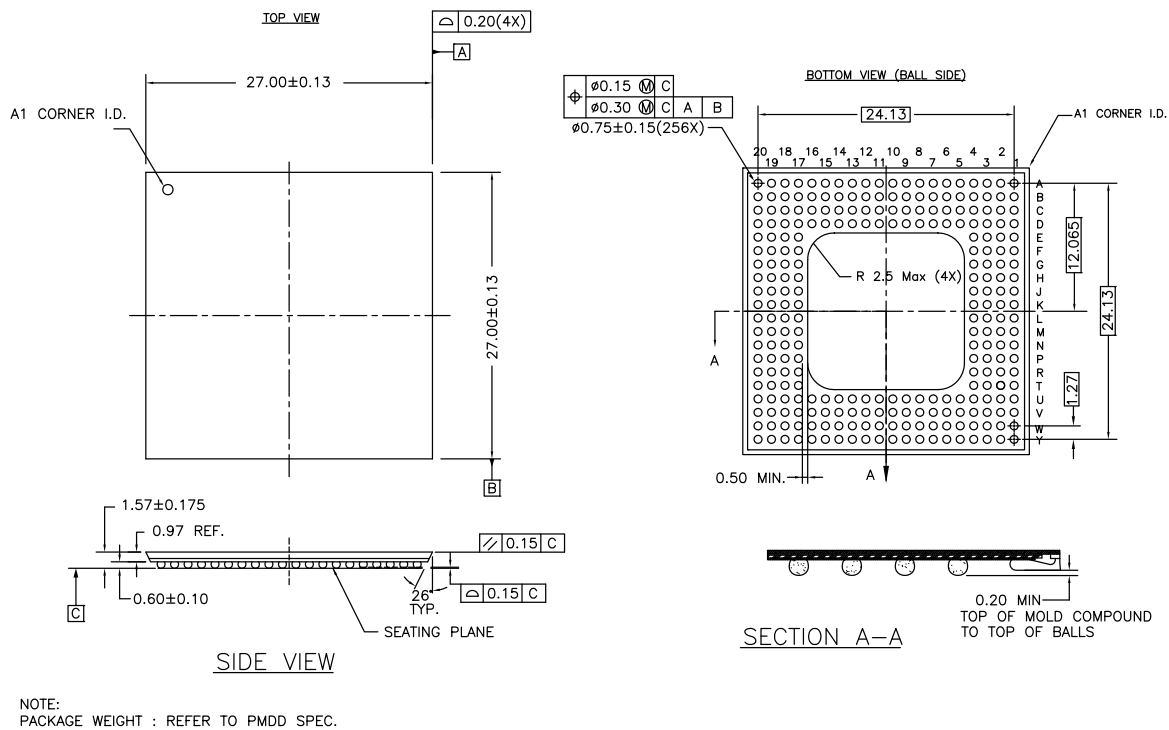
Figure 3. 256-pin L2 Ball Grid Array (27 × 27 × 1.57 mm) BJ256
