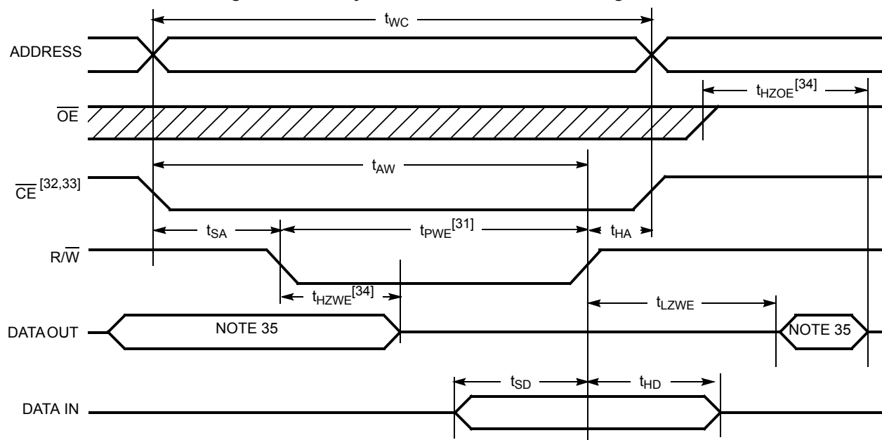
Figure 7. Write Cycle No. 1: \overline{R/\overline{W}} Controlled Timing [28, 29, 30, 31]
