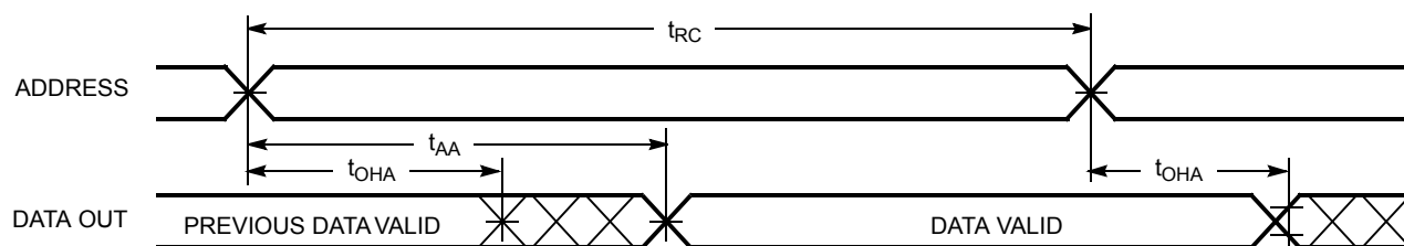
Figure 5. Read Cycle No. 2 (Either Port \overline{\text{CE}}/\overline{\text{OE}} Access) [23, 26, 27]
