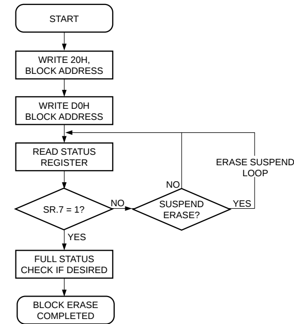
Figure 5 Block Erase Flowchart
