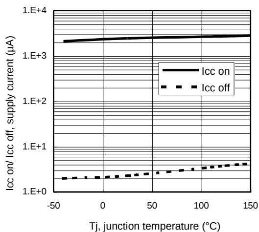
Figure 14 – Icc on/ Icc off (µA) Vs Tj (°C)
