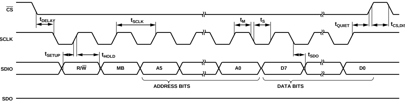
Figure 29. SPI 3-Wire Read/Write
