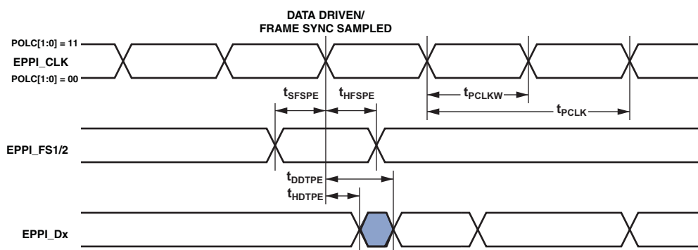
Figure 47. PPI External Clock GP Transmit Mode with External Frame Sync Timing
