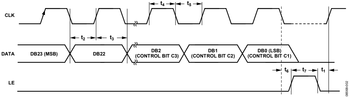
Figure 2. Timing Diagram
