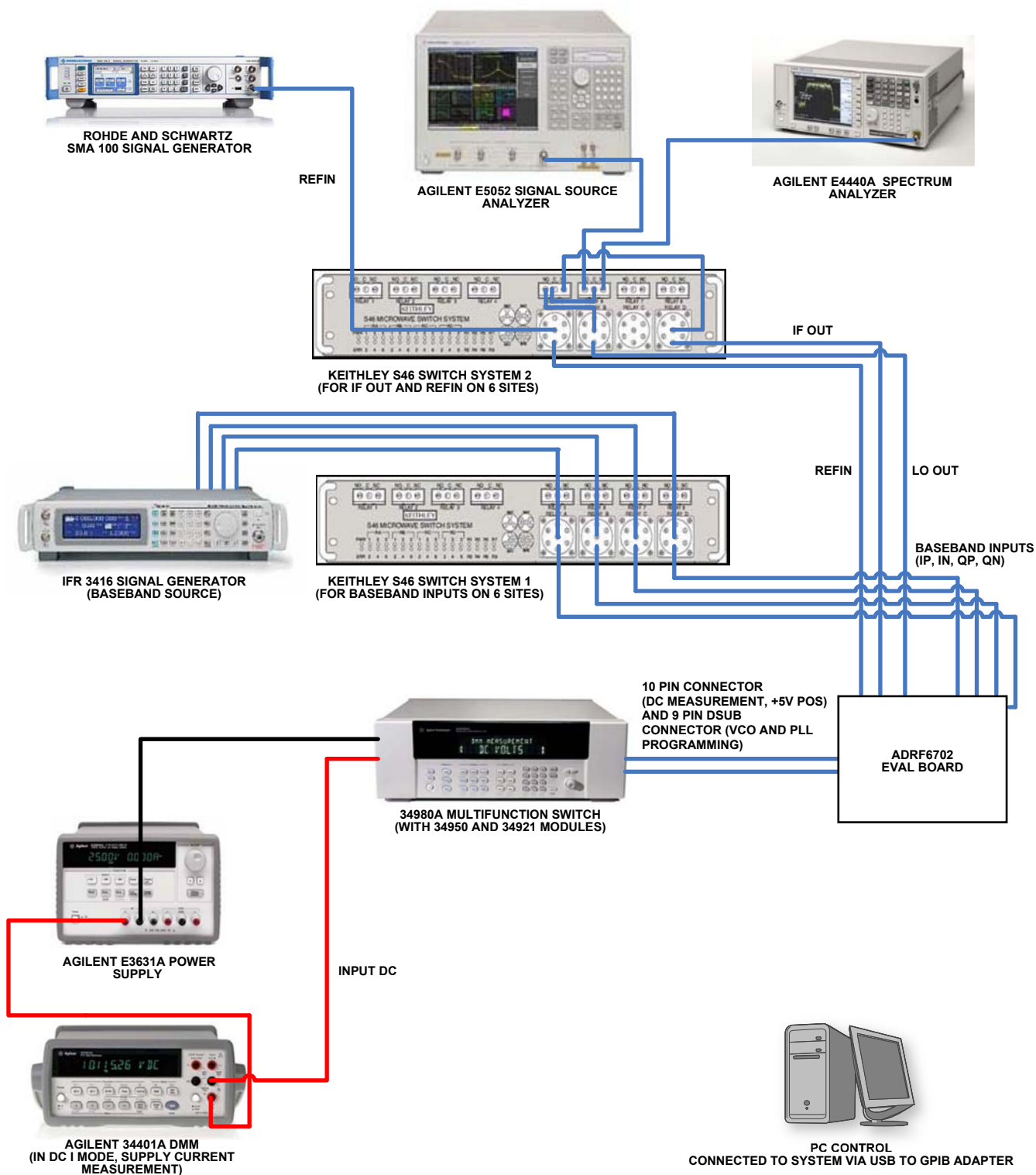
Figure 50. Characterization Setup for Phase Noise and Reference Spur Measurements
