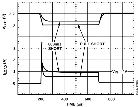
Figure 18. Short-Circuit Current
