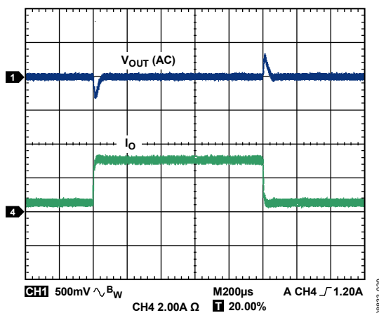
Figure 29. ADP2303 Load Transient, 0.5 A to 3.0 A, V_{OUT} = 5.0\text{ V} , V_{IN} = 12\text{ V} , L = 4.7\text{ μH} , C_{OUT} = 47\text{ μF}
