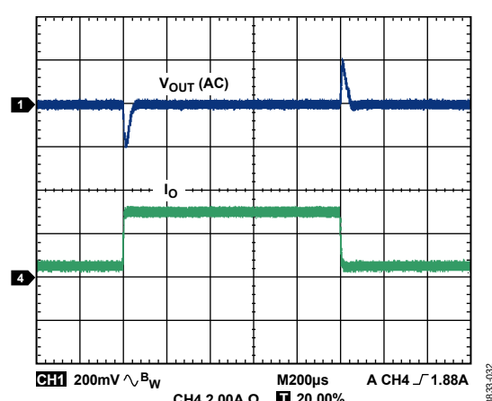
Figure 32. ADP2303 Load Transient, 0.5 A to 3.0 A, V_{OUT} = 3.3\text{ V} , V_{IN} = 12\text{ V} , L = 4.7\text{ μH} , C_{OUT} = 2 \times 47\text{ μF}
