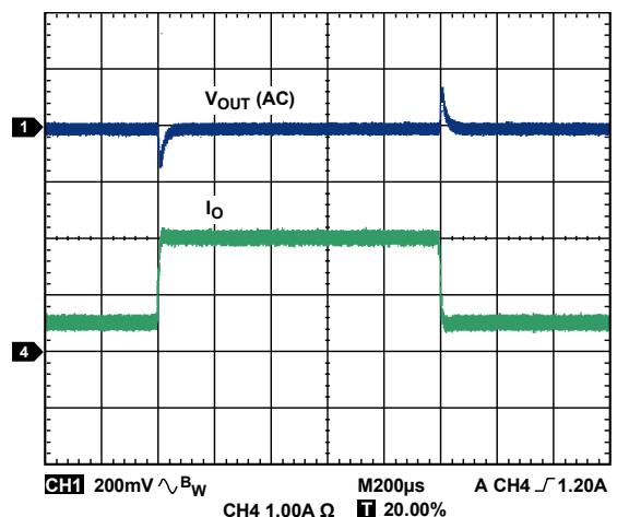
Figure 33. ADP2302 Load Transient, 0.5 A to 2.0 A, V_{OUT} = 3.3\text{ V} , V_{IN} = 12\text{ V} , L = 6.8\text{ μH} , C_{OUT} = 2 \times 22\text{ μF}
