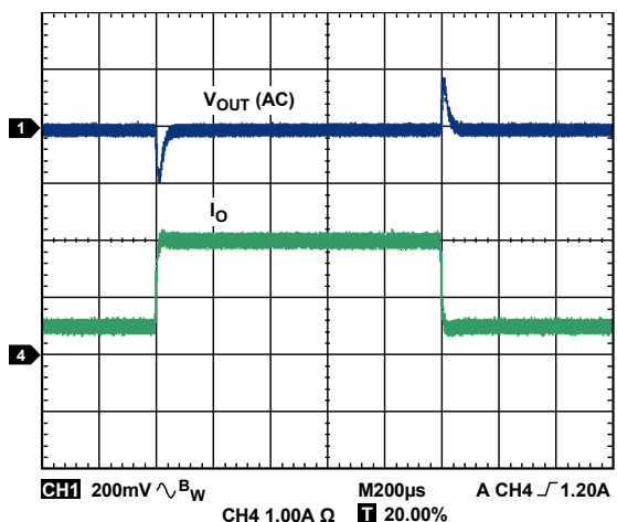
Figure 30. ADP2302 Load Transient, 0.5 A to 2.0 A, V_{OUT} = 5.0\text{ V} , V_{IN} = 12\text{ V} , L = 6.8\text{ μH} , C_{OUT} = 2 \times 22\text{ μF}
