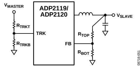
Figure 51. Voltage Tracking
