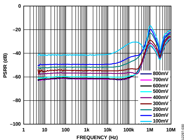
Figure 30. Power Supply Rejection Ratio (PSRR) vs. Frequency, V_{OUT} = 3\text{ V} , 500 mA Load Current, Various Headroom Voltages
