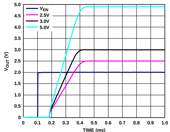
Figure 60. Typical Start-Up Behavior
