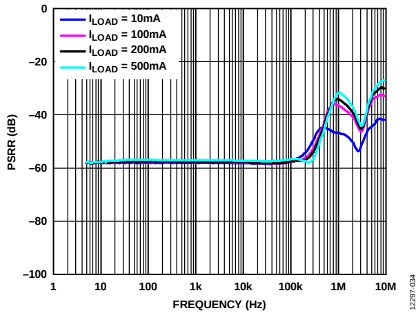
Figure 34. Power Supply Rejection Ratio (PSRR) vs. Frequency, 400 mV Headroom, V_{OUT} = 3\text{ V}
