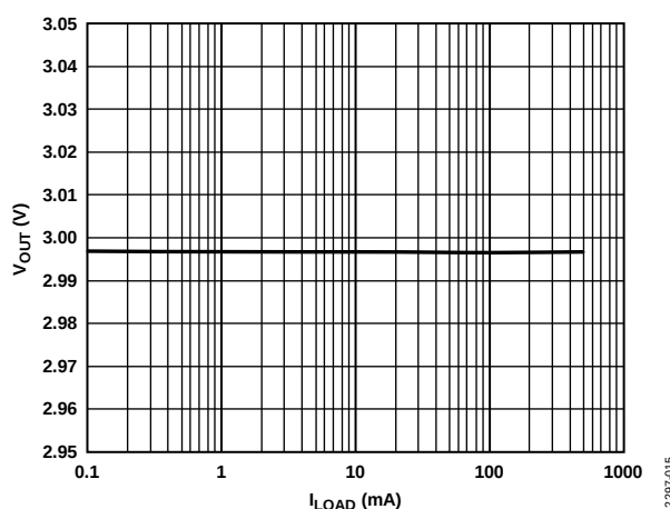
Figure 15. Output Voltage ( V_{OUT} ) vs. Load Current ( I_{LOAD} ), V_{OUT} = 3\text{ V}
