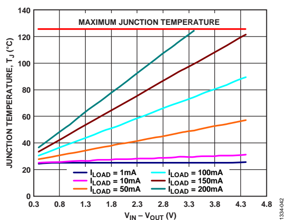
Figure 44. TSOT, 100 mm 2 of PCB Copper, T_A = 25^\circ\text{C}
