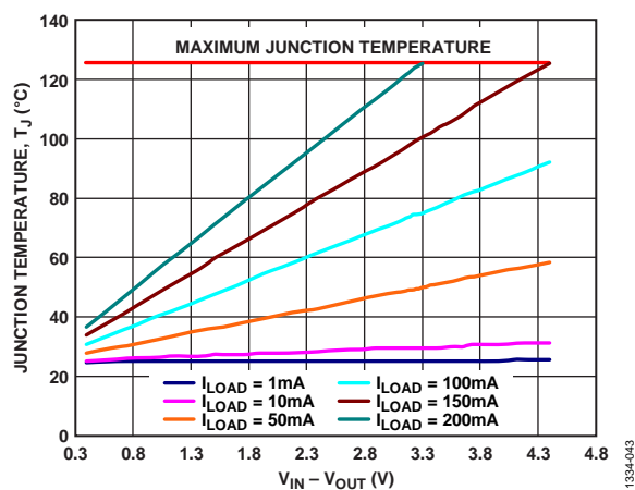
Figure 45. TSOT, 50 mm 2 of PCB Copper, T_A = 25^\circ\text{C}
