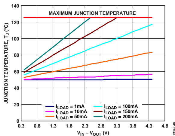
Figure 48. TSOT, 50 mm 2 of PCB Copper, T_A = 50^\circ\text{C}
