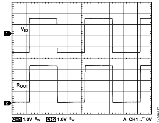
Figure 24. Receiver Propagation Delay (Oscilloscope Plot), Data Rate = 500 kbps, V_{ID} \geq 1.5 V
