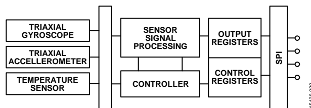
Figure 24. Basic Operation of the ADIS16475
