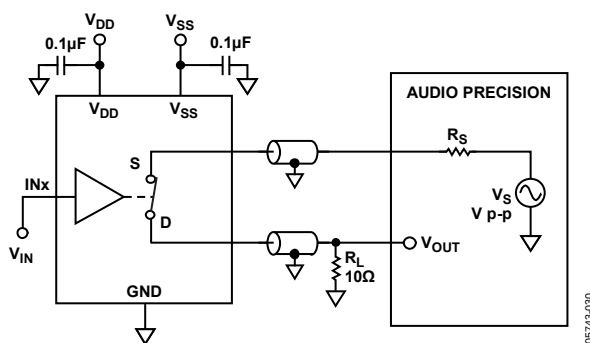
Figure 34. THD + Noise
