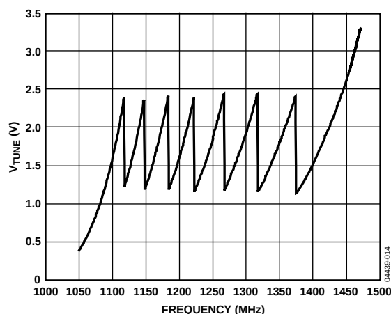
Figure 14. Frequency vs. V_{TUNE} , ADF4360-5
