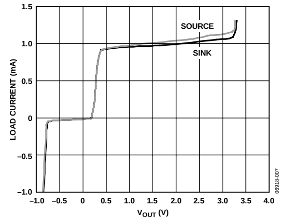
Figure 7. Load Current vs. V_{OH}/V_{OL}
