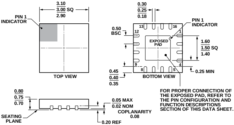
COMPLIANT TO JEDEC STANDARDS MO-220-WEED-6. Figure 22. 16-Lead Lead Frame Chip Scale Package [LFCSP_WQ] 3 mm × 3 mm Body, Very Very Thin Quad (CP-16-18) Dimensions shown in millimeters
