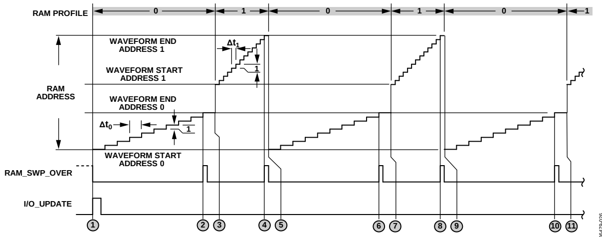
Figure 45. Internal Profile Control Timing Diagram (Continuous)
