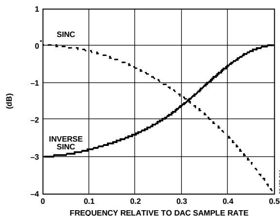
Figure 28. Sinc and Inverse Sinc Responses
