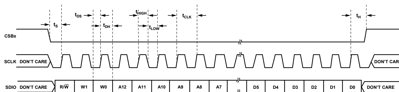
Figure 53. Serial Port Interface Timing Diagram
