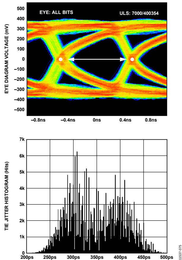
Figure 51. Data Eye for LVDS Outputs in ANSI-644 Mode with Trace Lengths of Less Than 24 Inches on Standard FR-4 Material, External 100 Ω Far End Termination Only
