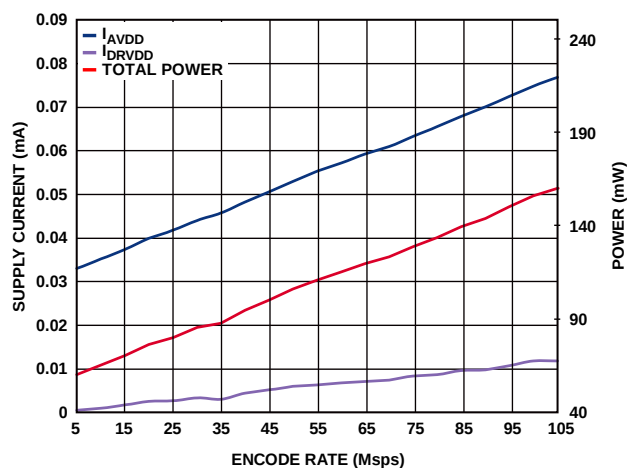
Figure 60. AD9608-105 Power and Current vs. Clock Rate (1.8 V CMOS Output Mode)
