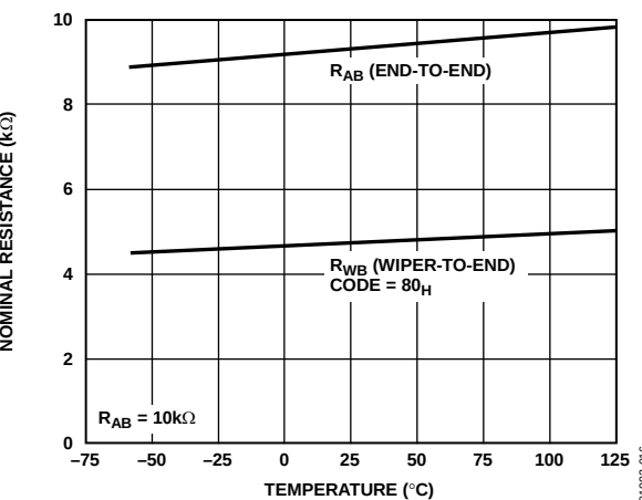
Figure 16. Nominal Resistance vs. Temperature
