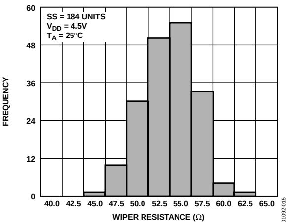
Figure 15. 100 kΩ Wiper-Contact-Resistance Histogram
