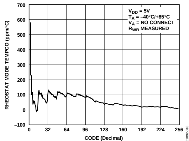
Figure 18. \Delta R_{WB}/\Delta T Rheostat Mode Tempco
