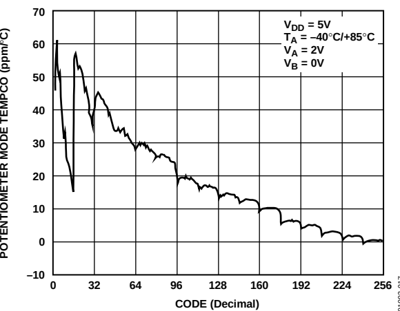
Figure 17. \Delta V_{WB}/\Delta T Potentiometer Mode Tempco
