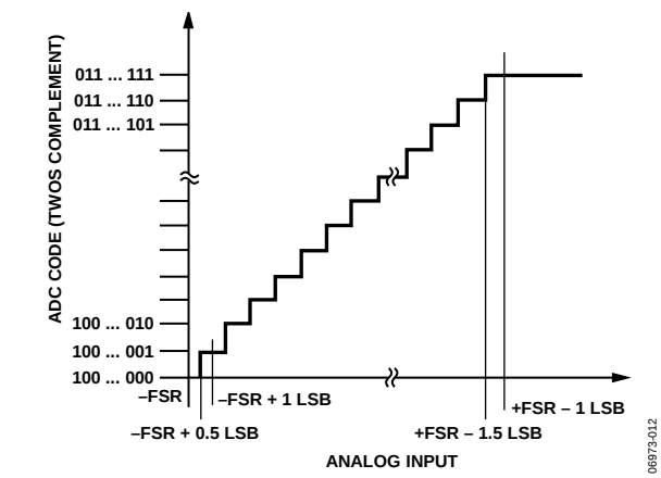
Figure 21. ADC Ideal Transfer Function
