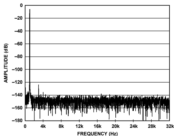
Figure 11. AD7766-1 FFT, 1 kHz, -6 dB Input Tone
