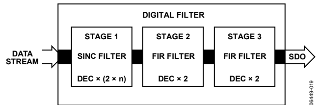
Figure 31. FIR Filter Stages
