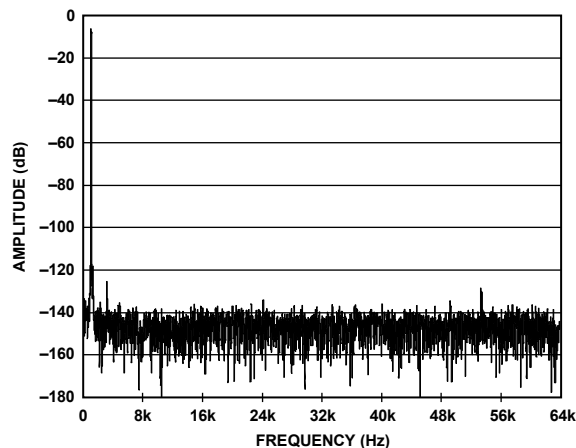
Figure 10. AD7766 FFT, 1 kHz, -6 dB Input Tone
