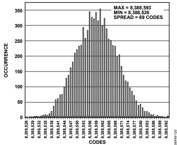
Figure 25. AD7766-2 24-Bit Histogram
