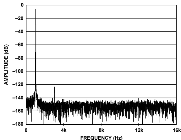
Figure 12. AD7766-2 FFT, 1 kHz, -6 dB Input Tone
