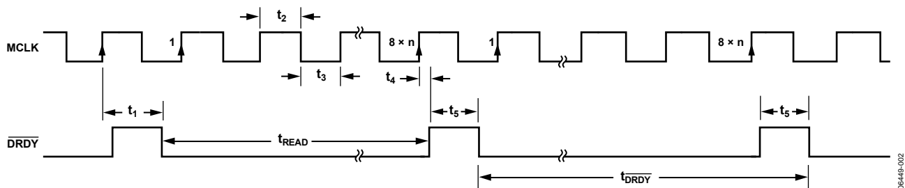
Figure 2. \overline{\text{DRDY}} vs. MCLK Timing Diagram, n = 1 for AD7766 (Decimate by 8), n = 2 for AD7766-1 (Decimate by 16), n = 4 for AD7766-2 (Decimate by 32)
