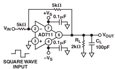
TPC 23a. Unity Gain Inverter
