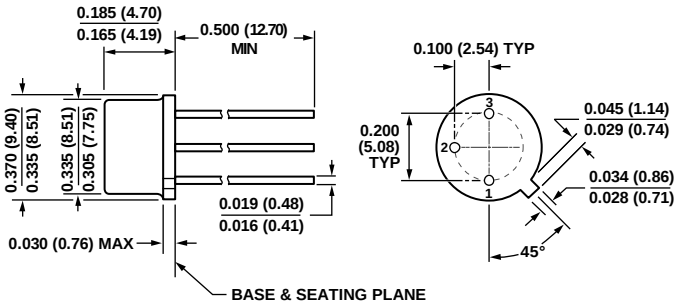
Figure 17. 3-Pin Metal Header Package [TO-5] (H-03B)
