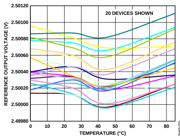
Figure 43. Reference Output Voltage vs. Temperature ( 0^{\circ}\text{C} to +85^{\circ}\text{C} )
