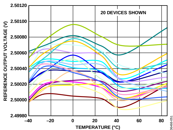
Figure 42. Reference Output Voltage vs. Temperature ( -40^{\circ}\text{C} to +85^{\circ}\text{C} )
