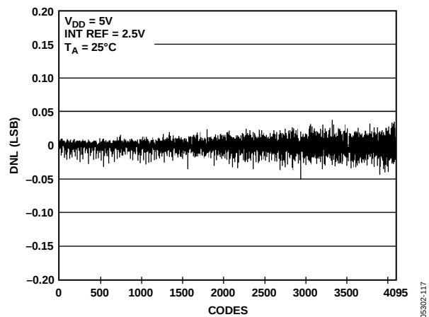
Figure 18. DNL AD5628-2
