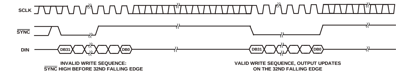
Figure 60. \overline{\text{SYNC}} Interrupt Facility
