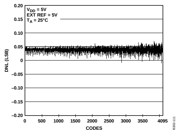
Figure 12. DNL AD5628—External Reference
