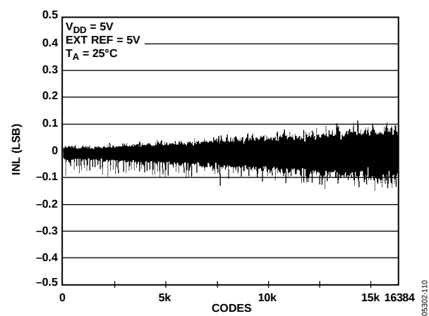
Figure 11. DNL AD5648—External Reference
