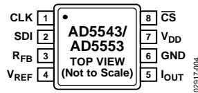
Figure 6. Pin Configuration
