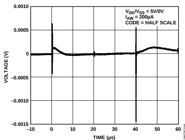
Figure 34. Digital Feedthrough
