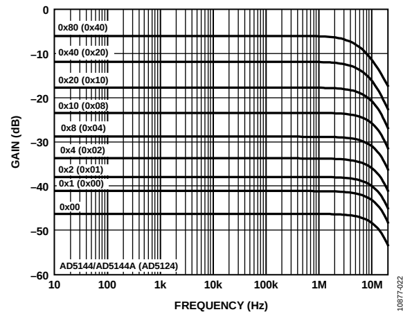
Figure 25. 10 \text{ k}\Omega Gain vs. Frequency vs. Code
