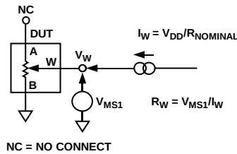
Figure 41. Wiper Resistance
