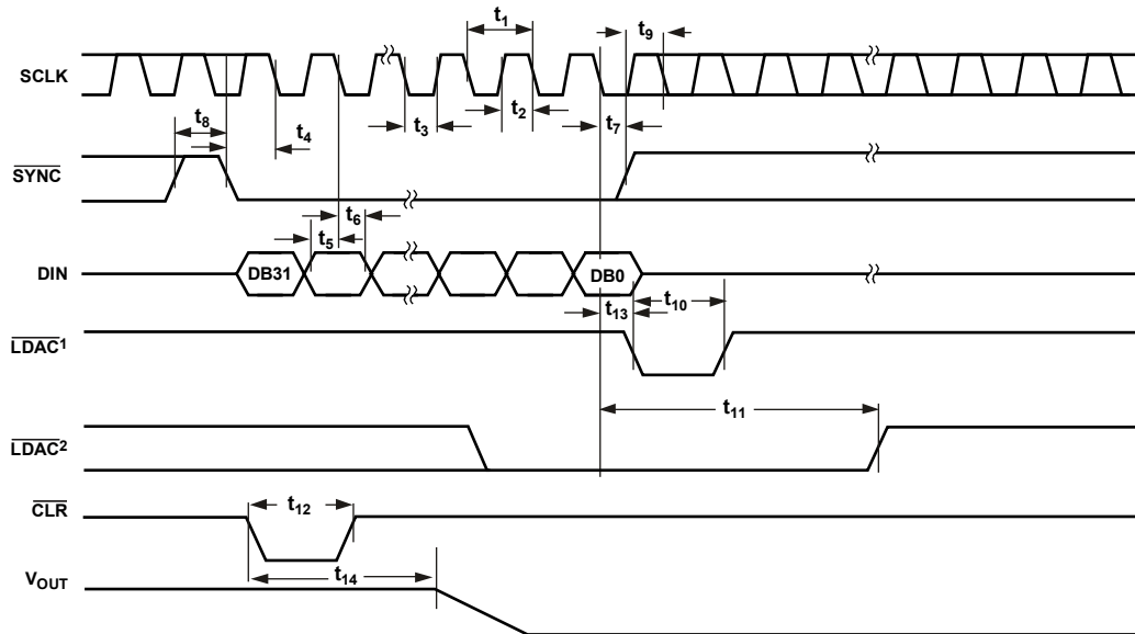
Figure 4. Serial Write Operation
