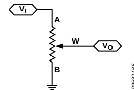
Figure 48. Potentiometer Mode Configuration
