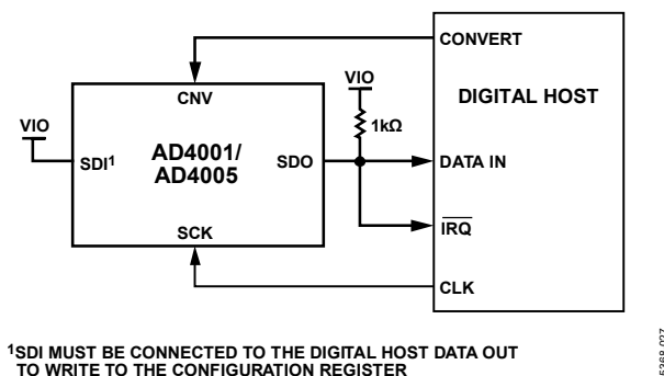
Figure 56. CS Mode, 3-Wire with Busy Indicator Connection Diagram
