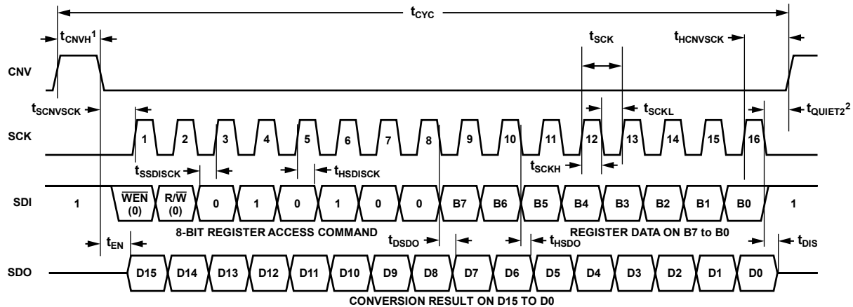
Figure 49. Register Write Timing Diagram
