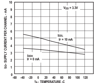
Figure 25: Typical Supply Current per Channel vs. Temperature for 3.3V Operation
