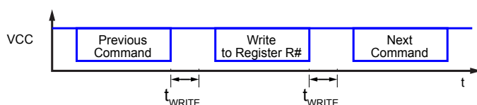
Figure 14: Writing to Volatile Memory
